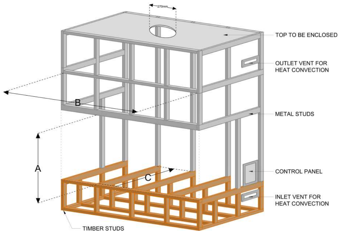
Figure 1.9 (Metal framing)
