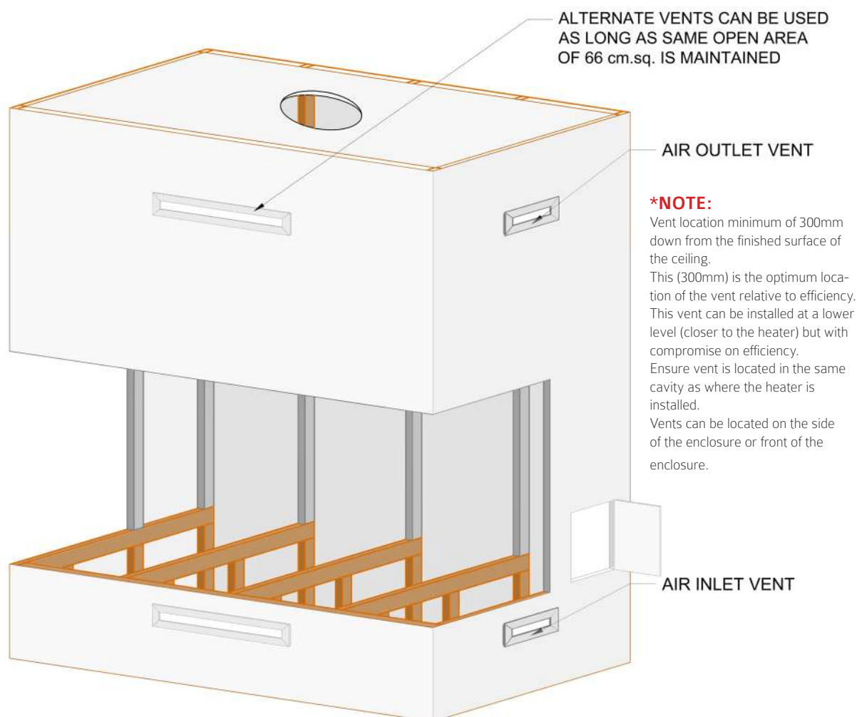
Figure 1.2 (Vents)
