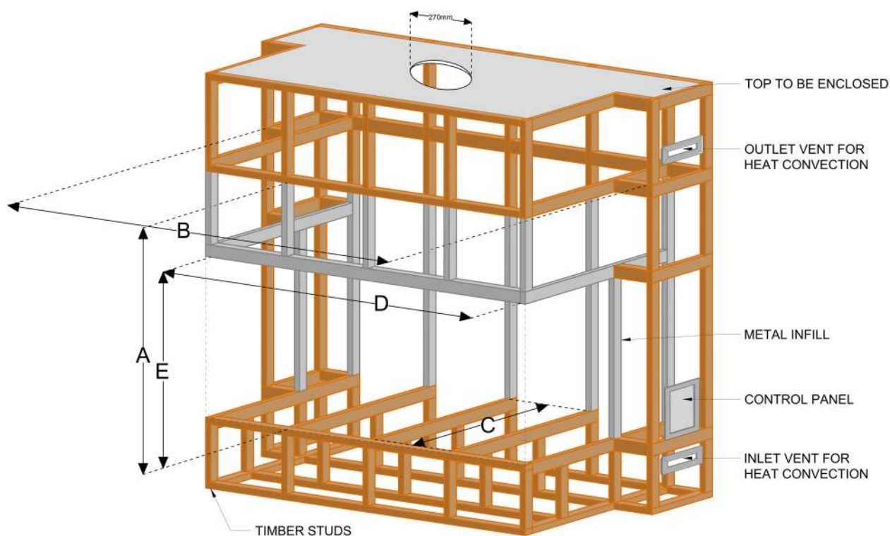
Figure 1.8 (Timber framing)
